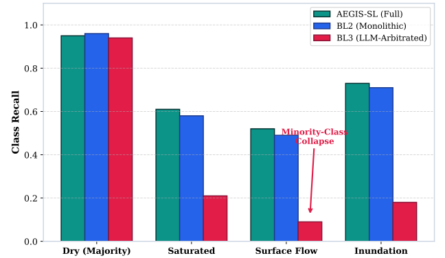
Figure 5: Per-Class Recall & LLM Minority-Class Collapse Diagnostic (H2). Grouped recall comparison across flood classes. Prompt-chained LLM arbitration (BL3) collapses on minority classes (saturated 0.21, surface 0.09, inundation 0.18), whereas AEGIS-SL maintains strong recall across all states.
